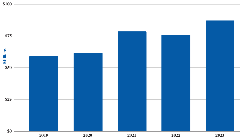
Net Assets
